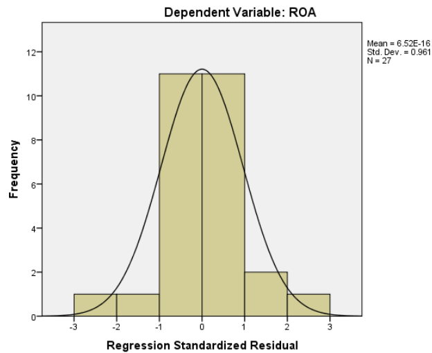
Gambar 4.1 Histogram
